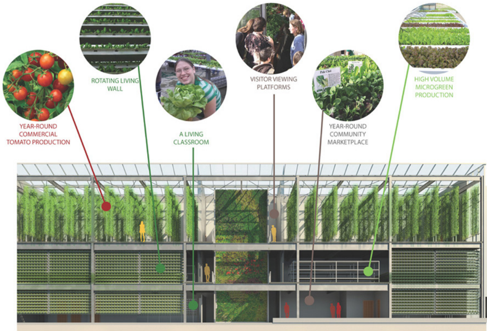
RENDERED LONGITUDINAL AND CROSS-SECTION
